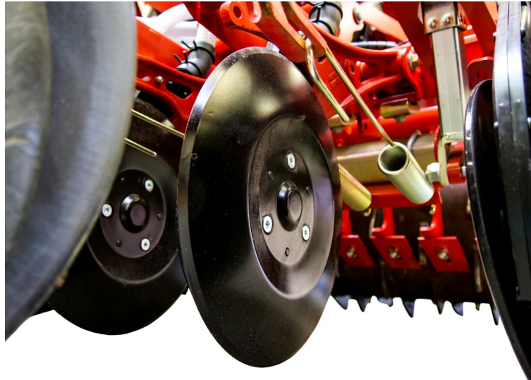
Kverneland f-drill CB F new bolted CX-II coulters without press wheel
