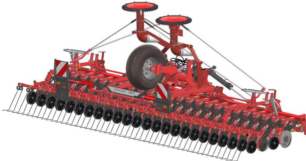
Kverneland f-drill CB F, folding coulters with two distribution heads for double-entry system
